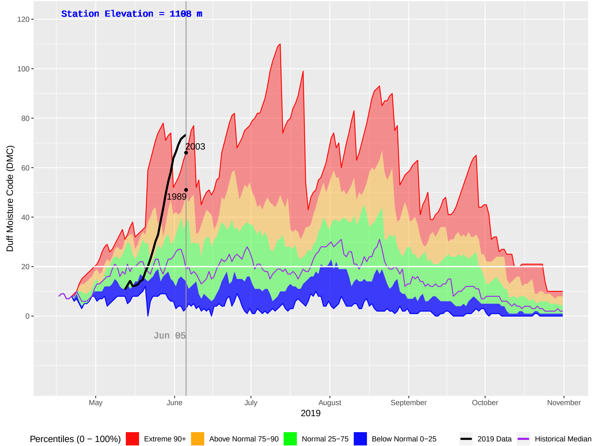
NABESHE (151) : Historical (1987–2018), Current (2019) Daily Duff Moisture Code (DMC)
