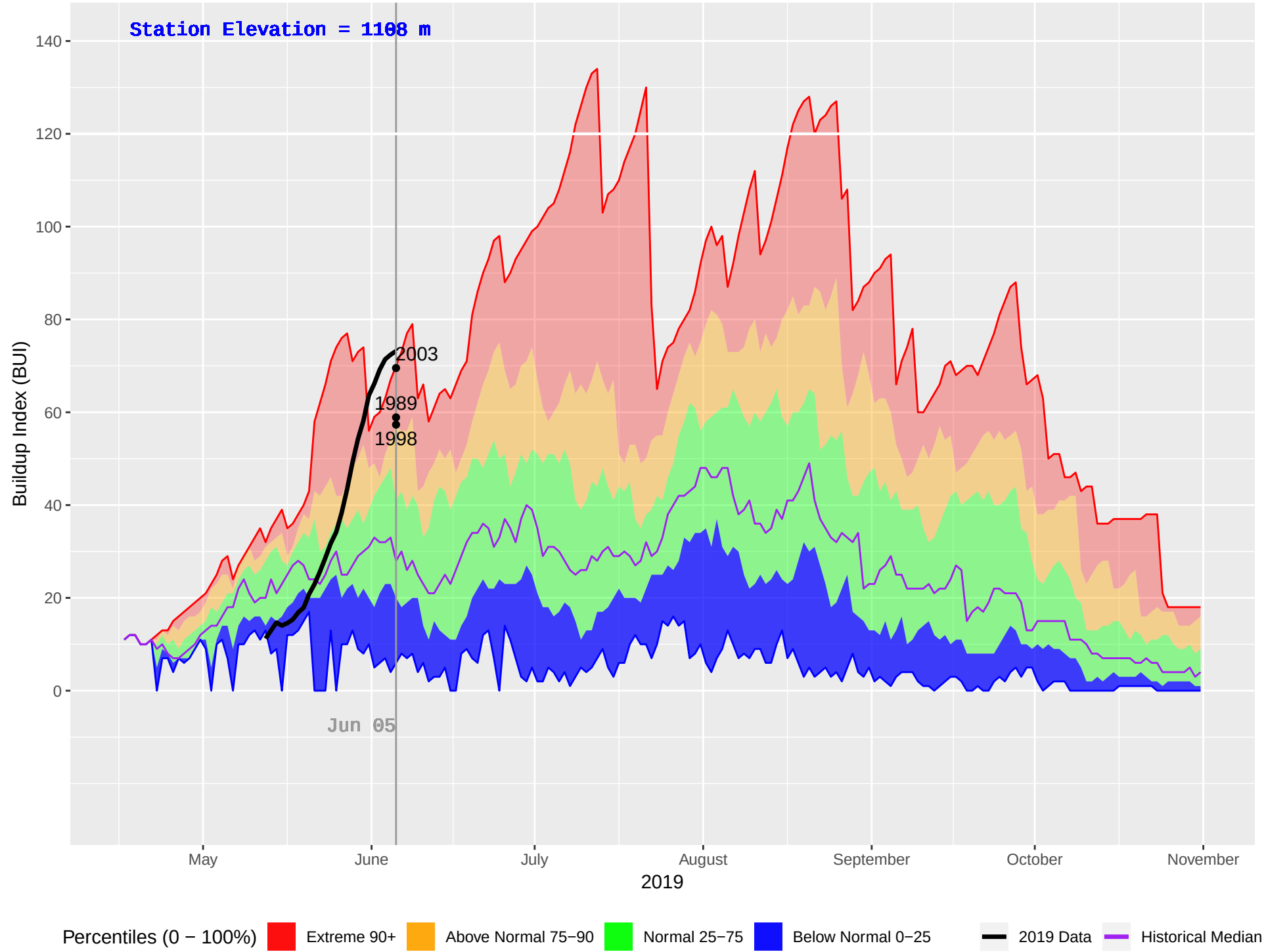
NABESHE (151) : Historical (1987–2018), Current (2019) Daily Buildup Index (BUI)
