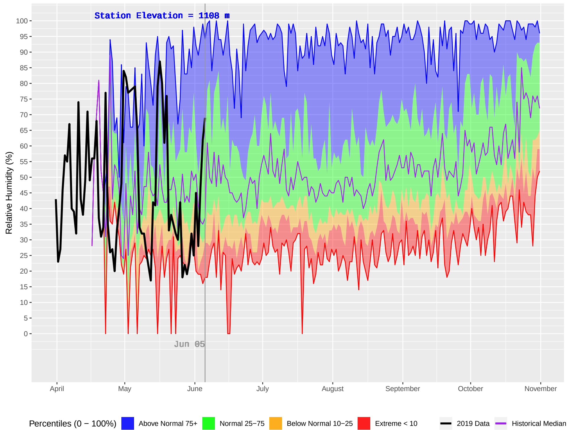
NABESHE (151) : Historical (1987–2018) and Current (2019) Daily Relative Humidity
