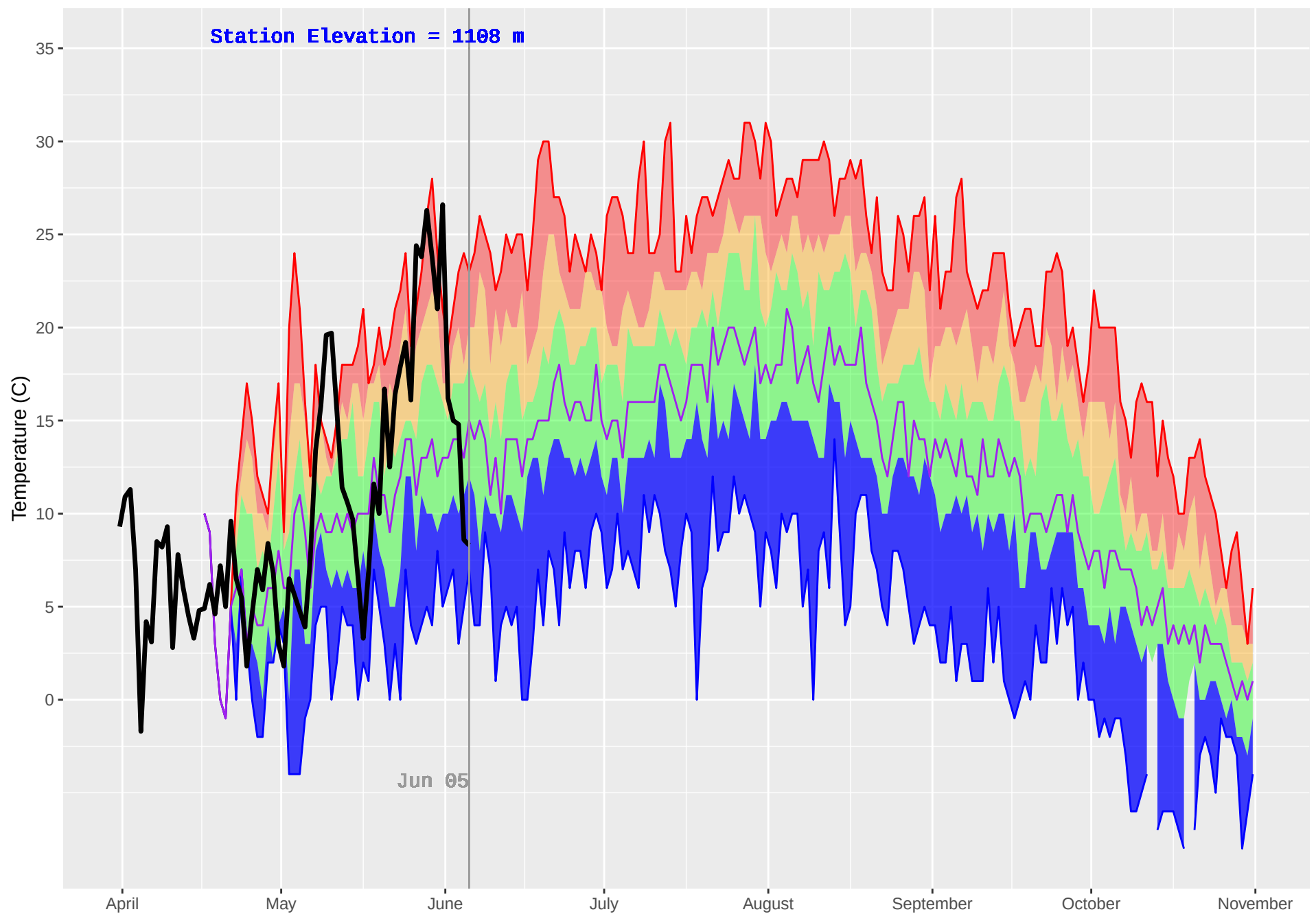
NABESHE (151) : Historical (1987–2018) and Current (2019) Daily Temperature
