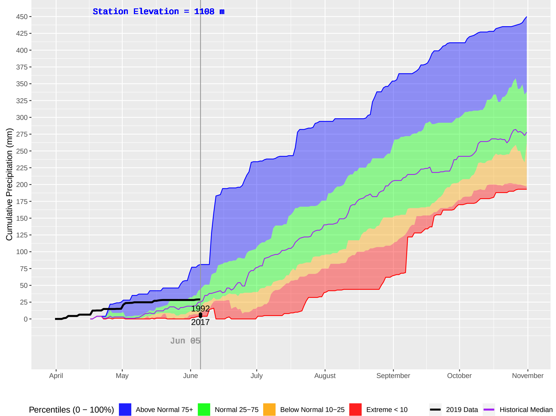
NABESHE (151) : Historical (1987–2018), Current (2019) Daily Cumulative Precipitation
